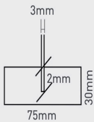
Snaprex wood base with notch, solid wood untreated without panel.
